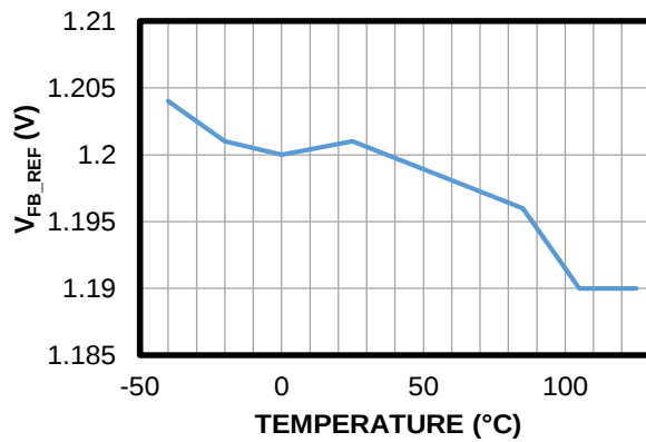
V_{FB} Reference vs. Temperature
