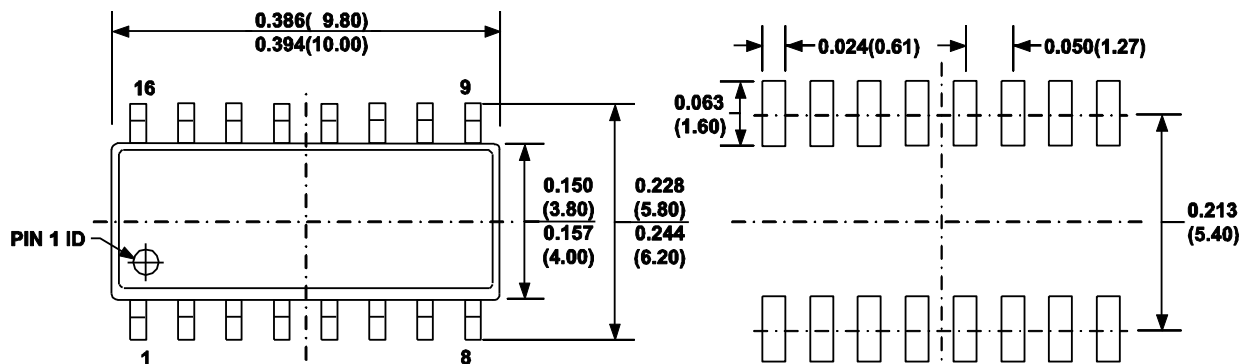
TOP VIEW
