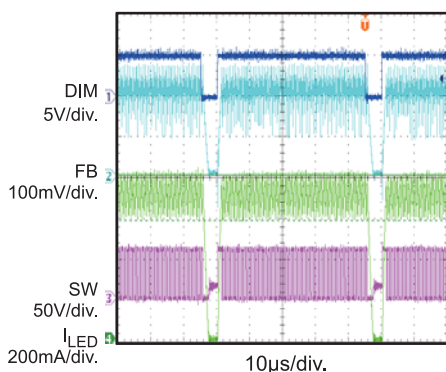
PWM Dimming
