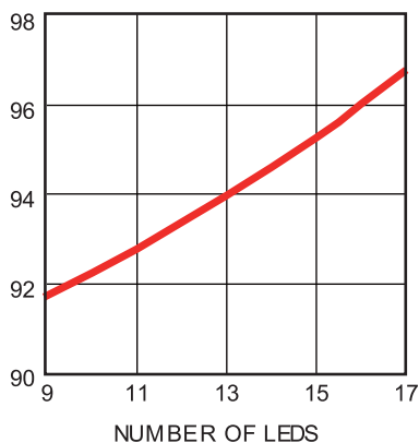
Efficiency vs. LED number
