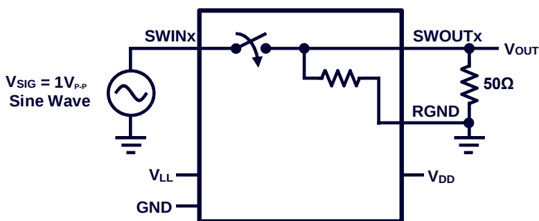
Figure 9: Test Circuit 8
