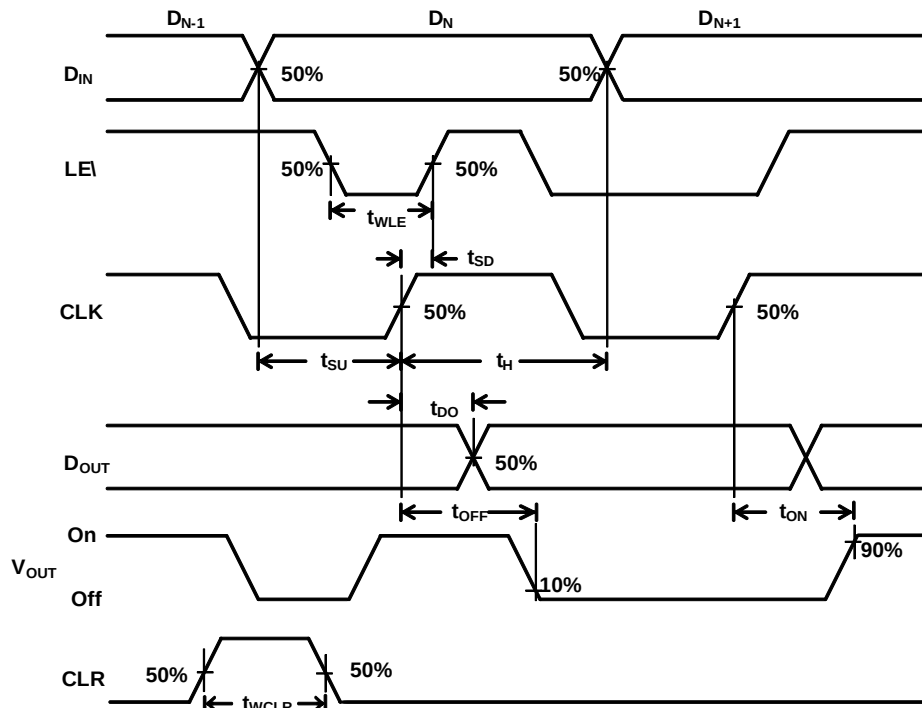
Figure 1: Timing Diagram
