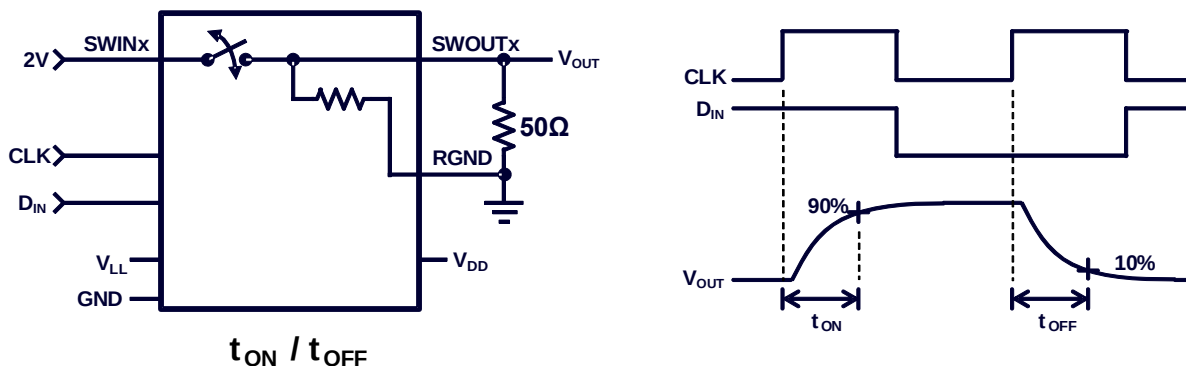
Figure 5: Test Circuit 4
