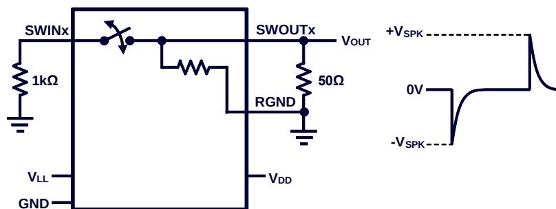
Figure 8: Test Circuit 7
