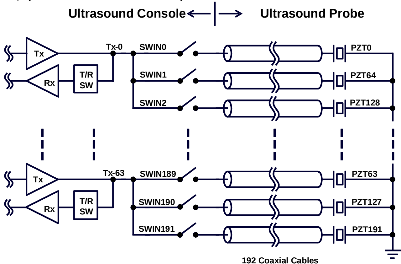
Figure 16: The MP4833A in an Ultrasound Console
