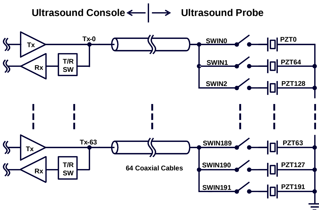
Figure 17: The MP4833A inside the Ultrasound Probe Head
