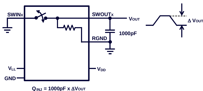
Figure 9: Test Circuit 8
