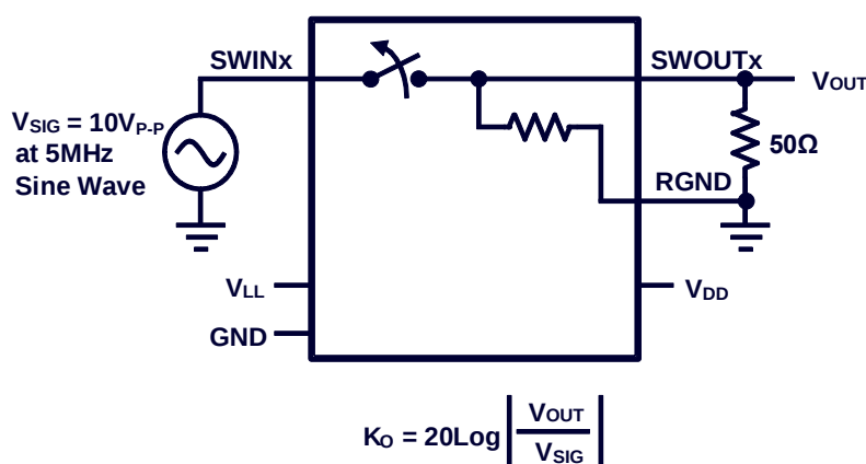
Figure 6: Test Circuit 5
