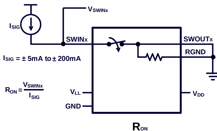
Figure 2: Test Circuit 1
