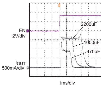
Inrush Current with Different Load Capacitance
