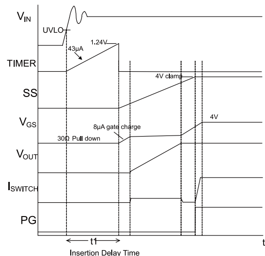
Figure 4: Start-Up Sequence
