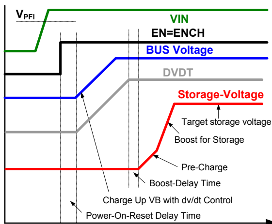
Figure 2: Charging Process
