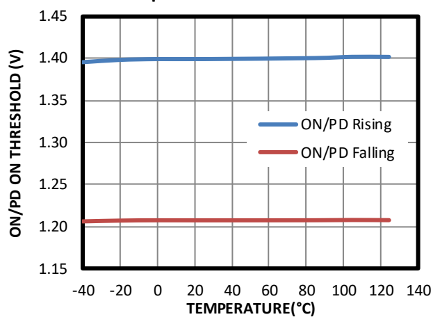
ON/PD FET On/Off Threshold vs. Temperature
