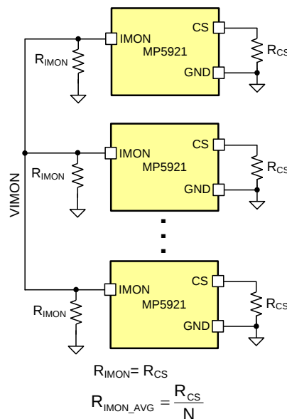
Figure 12: Multi-MP5921 IMON and CS Connection in Parallel Application
