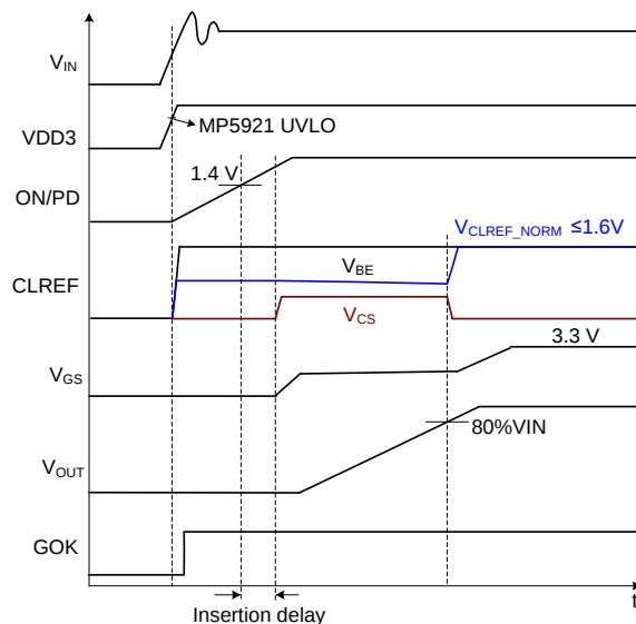
Figure 6: Start-Up when MP5921 Operates in Standalone Mode
