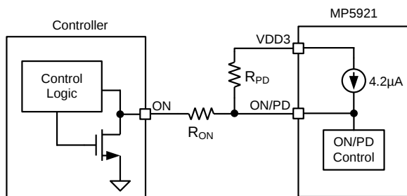
Figure 9: ON/PD Connection for PD Mode
