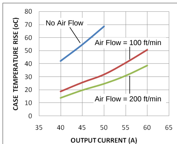
Figure 13: Output Current De-Rating Curve
