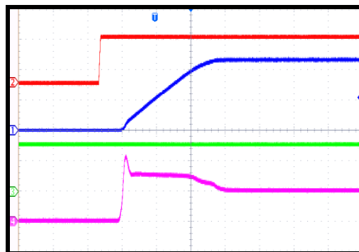
Start-Up through ON/PD
