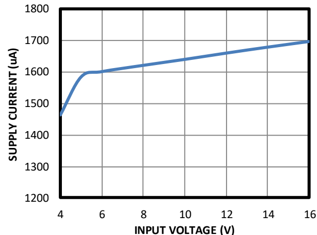
Supply Current vs. Input Voltage ON/PD = High
