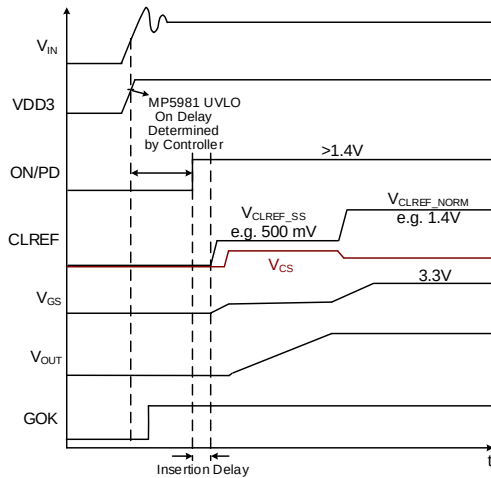
Figure 4: Start-Up when the MP5981 is Controlled by a Hot-Swap Controller
