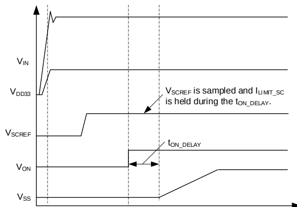
Figure 13: SCREF Voltage Sampling to Determine the Short-Circuit Current Limit
