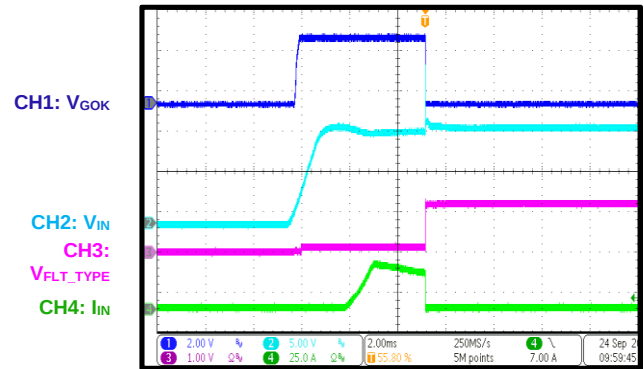
Short-Circuit Start-Up
