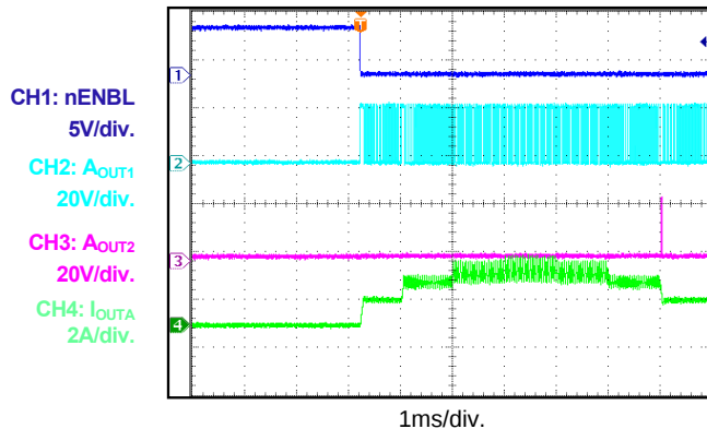
Enable, Quarter-Step
