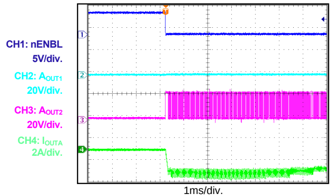
Enable, Eighth-Step
