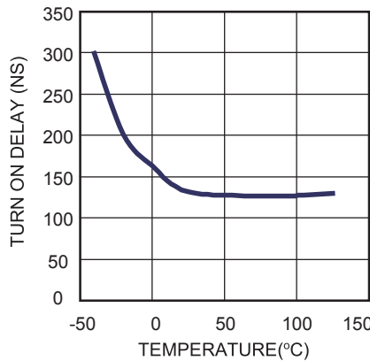
Turn On Delay (Cload=10nF) vs. Temperature
