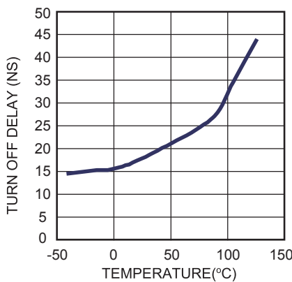
Turn Off Delay (Cload=10nF) vs. Temperature
