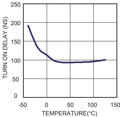
Turn On Delay (Cload=5nF) vs. Temperature
