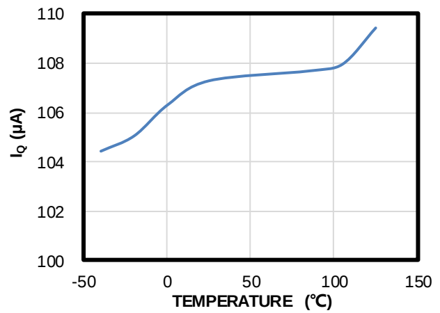
Quiescent Current vs. Temperature ( V_{DD} = 7V )
