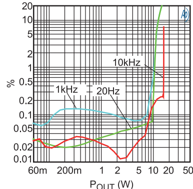
THD+N vs. POUT (12V, 6Ω)
