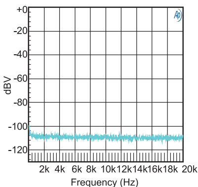
FFT Noise Floor Test (18V, 8Ω)
