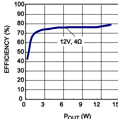
Efficiency vs. POUT 4Ω + 33μH
