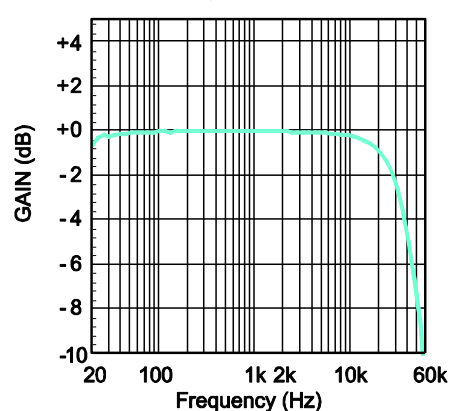
Frequency Response 12V, 4Ω + 33μH, 1W
