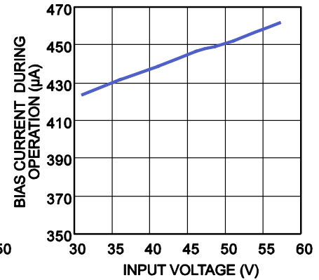
Bias Current during Operation vs. Input Voltage
