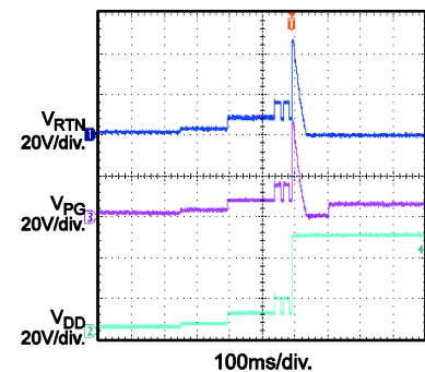
Start-Up by PSE
