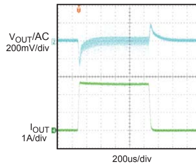
Transient Response
