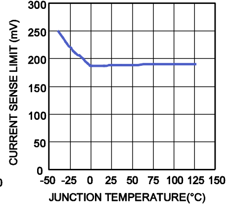
Flyback Controller Current Sense Limit vs. Junction Temperature
