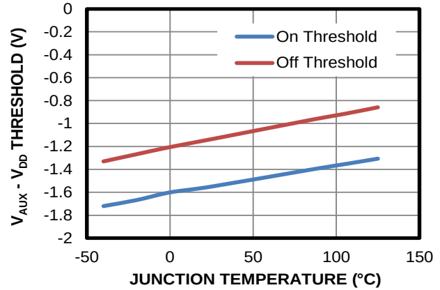
V_{AUX} - V_{DD} vs. Junction Temperature
