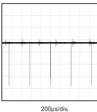
BS Recharge Cycling ( V_{DD} = 19V , R_L = 16\Omega )
