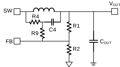
Figure 11: Simplified Circuit with External Ramp Compensation
