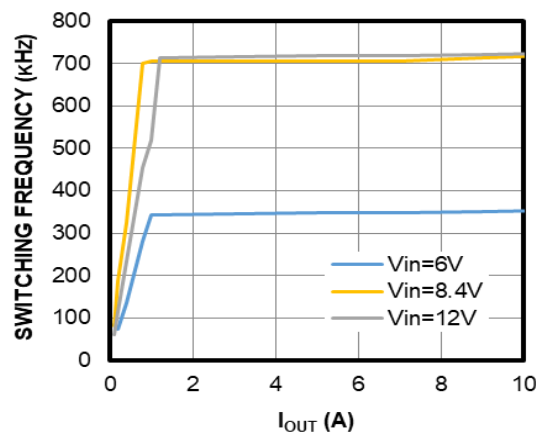
Switching Frequency vs. IOUT
