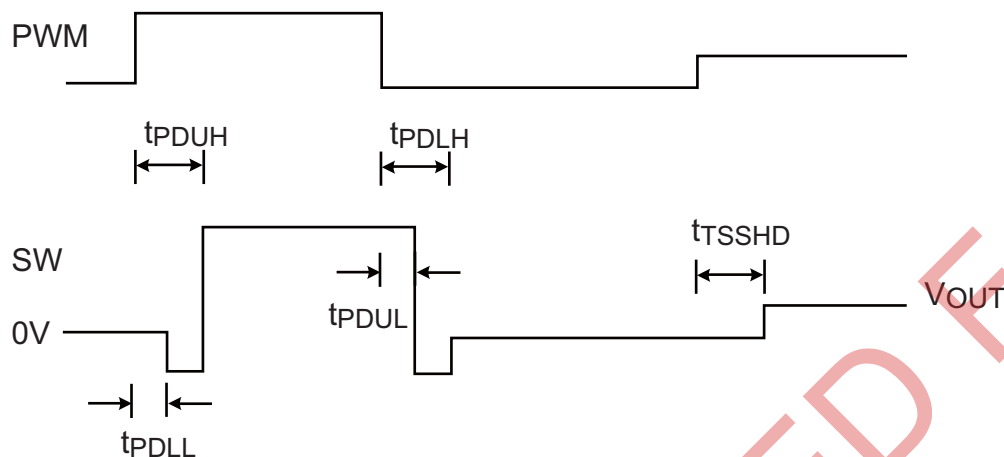
Figure 1- Timing Diagram
