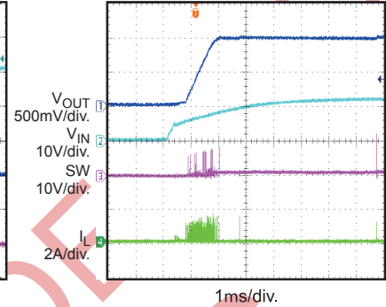
Start Up Through V_{IN} I_{OUT} = 0A
