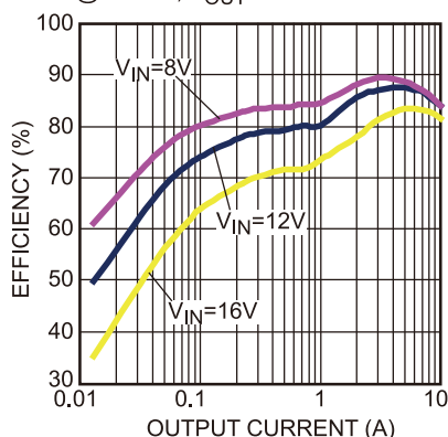
Figure 16 — Efficiency Curve
