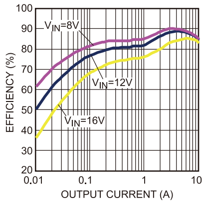
Figure 28 — Efficiency Curve
