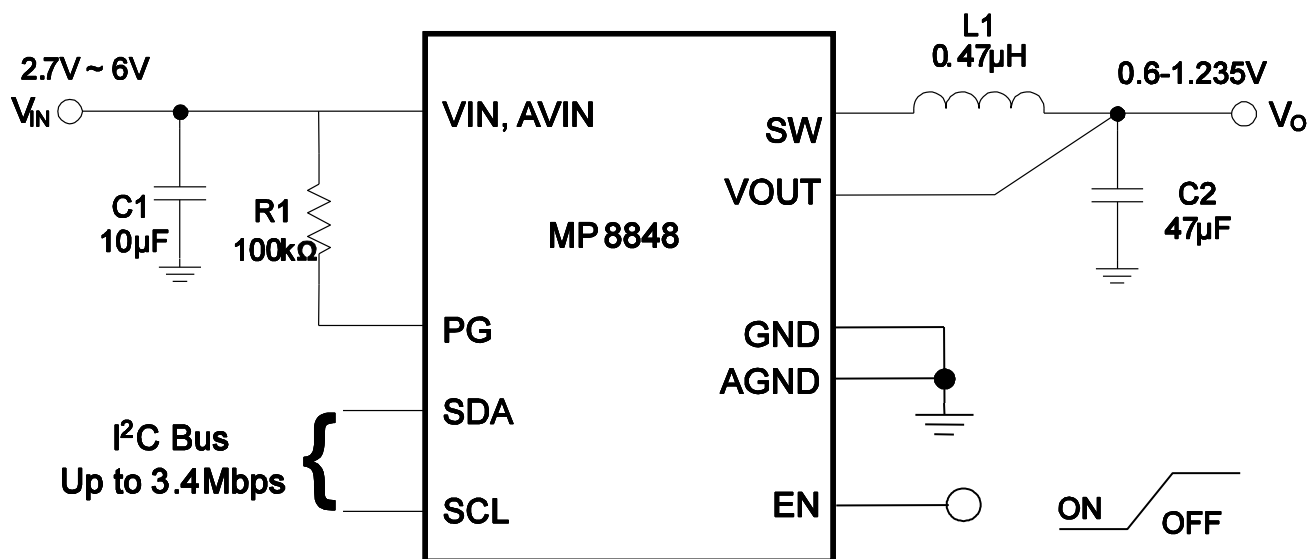
Figure 3: Application Circuit
