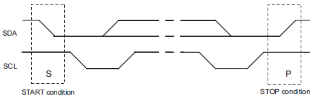
Figure 10: Start and Stop Condition
