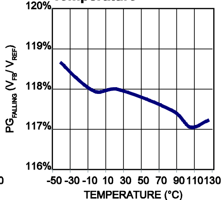
PG Falling Threshold ( V_{FB} Rising) vs. Temperature
