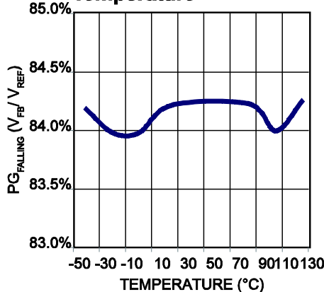
PG Falling Threshold ( V_{FB} Falling) vs. Temperature
