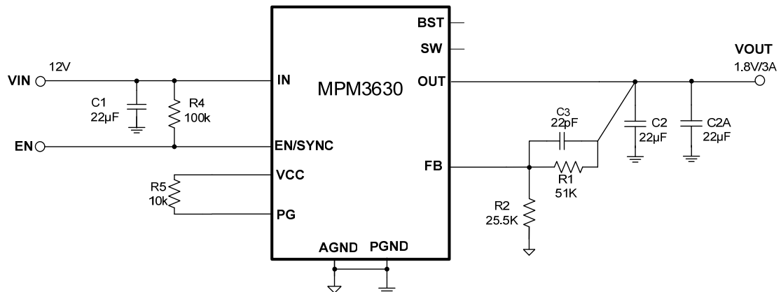
Figure 12: V_o = 1.8V , I_o = 3A
