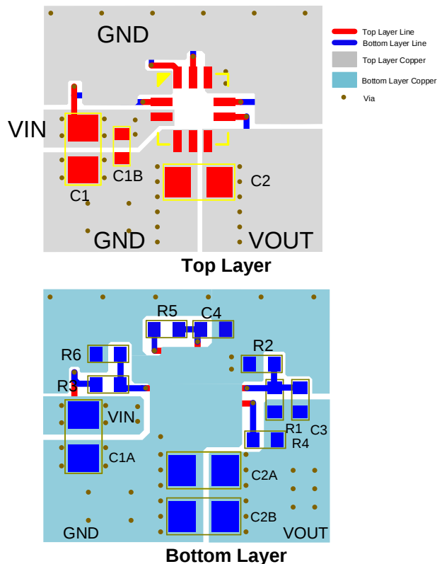
Figure 6: Recommended Layout
