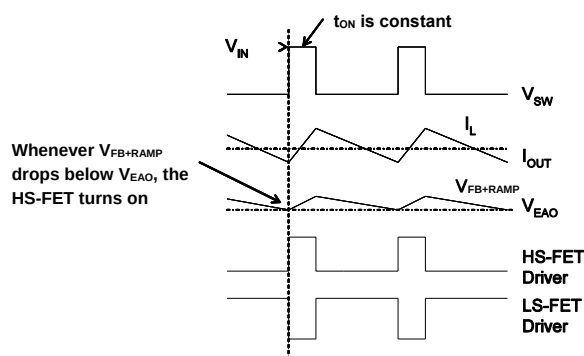
Figure 3: FCCM Operation
