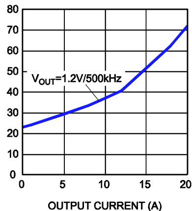
Thermal Results T_{ambient}=22^{\circ}C
