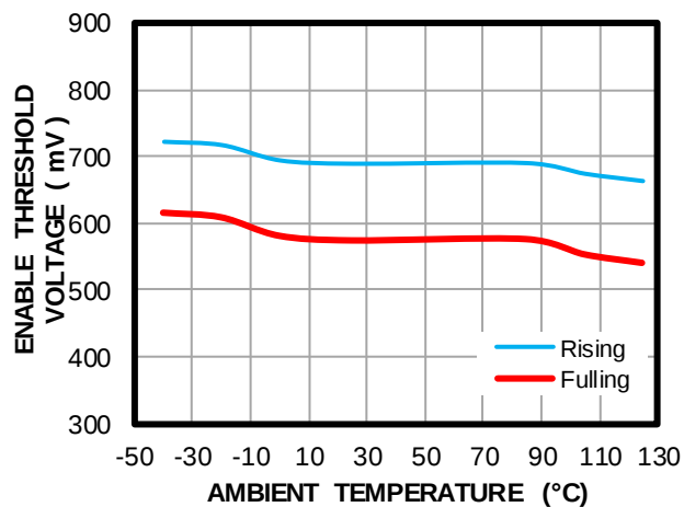
Enable Threshold Voltage vs. Temperature
