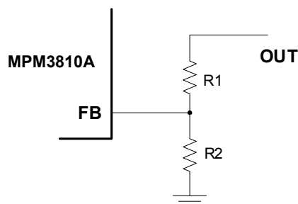
Figure 2: Feedback Network
