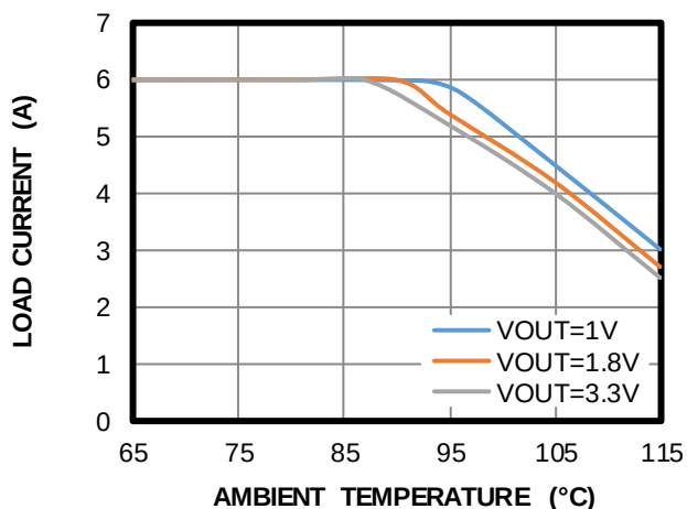
Thermal Derating
