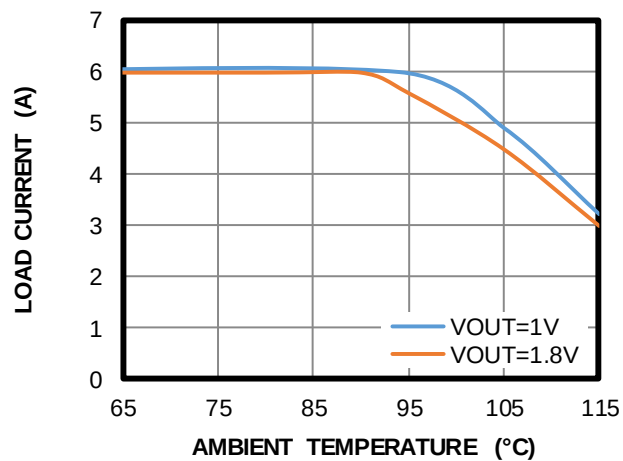
Thermal Derating
