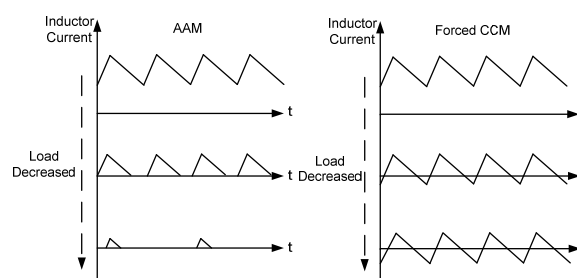
Figure 3: AAM and Forced CCM
