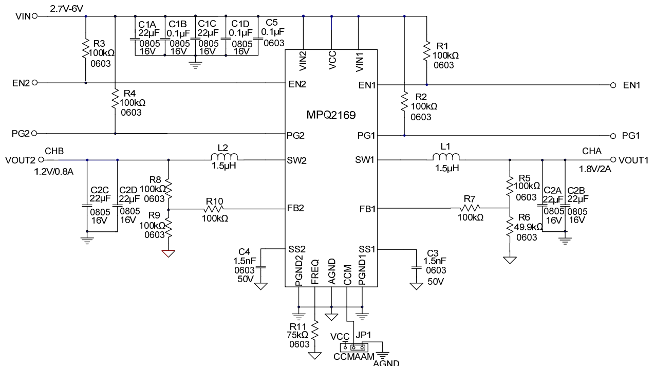
Figure 8 : 2A/0.8A Application Circuit
