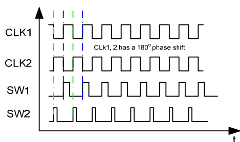
Figure 2: 180° Out-of-Phase Operation
