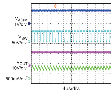
Analog Dimming
