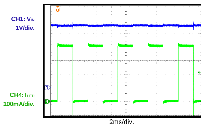
PWM Dimming
