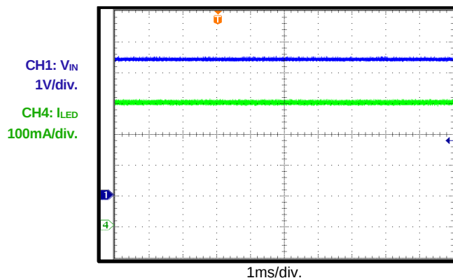
Steady State
