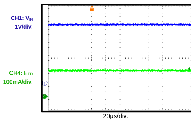
Analog Dimming
