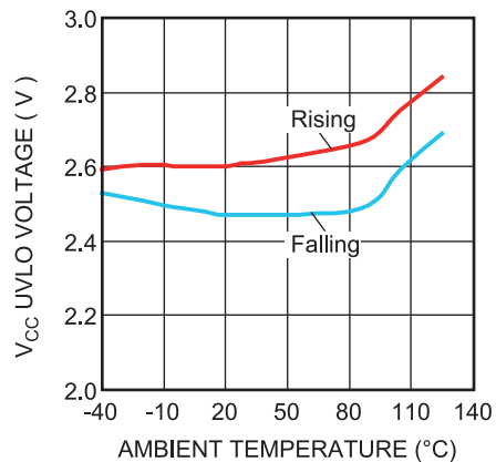
V_{CC} UVLO Voltage vs. T_A
