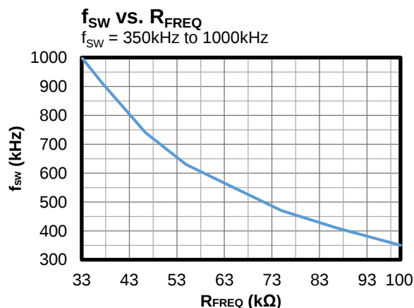
Figure 5: f sw vs. R FREQ
