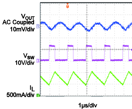
Output Voltage Ripple I_{OUT}=0.75A
