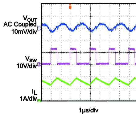
Output Voltage Ripple I_{OUT}=1.5A
