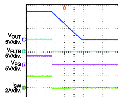
Thermal Shutdown
