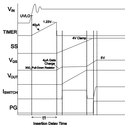
Figure 4: Start-Up Sequence
