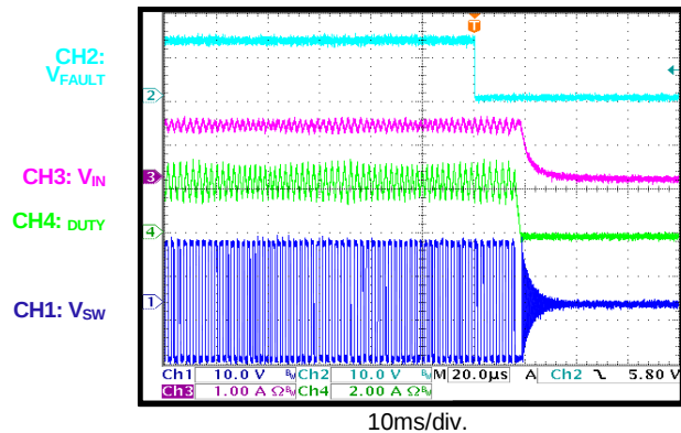
FAULT Short after VIN Start-Up
