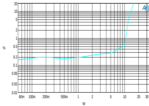
THD + N vs. P_{OUT} 8Ω + 66μH
