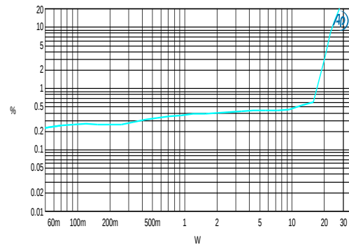
THD + N vs. P_{OUT} 4Ω + 33μH
