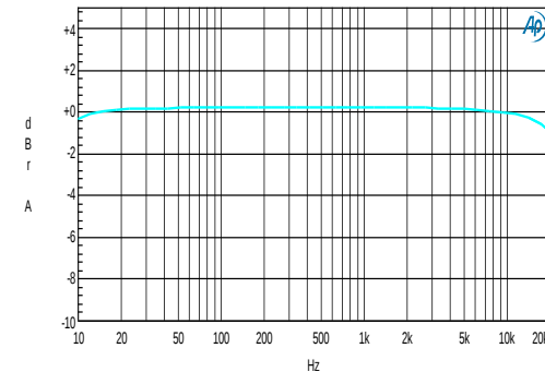
Frequency Response 1W, 4Ω + 33μH
