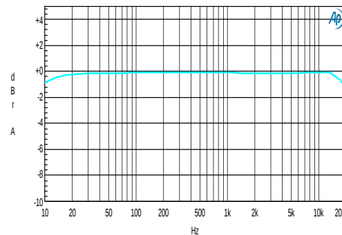
Frequency Response
