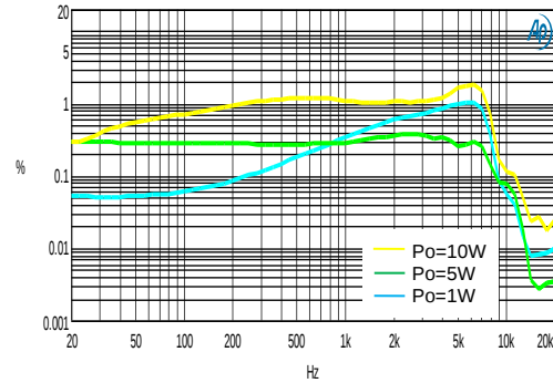
THD + N vs. Frequency 4Ω + 33μH
