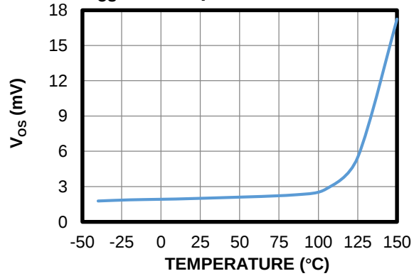
V_{OS} vs. Temperature
