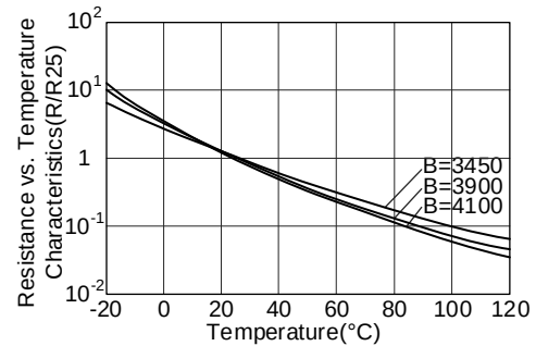
Figure 19: NTC Resistance vs. Temperature
