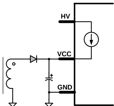
Figure 13: Start-Up Circuit
