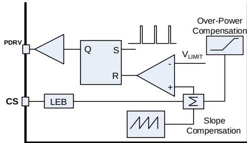
Figure 15: Peak Current Comparator Circuit Logic
