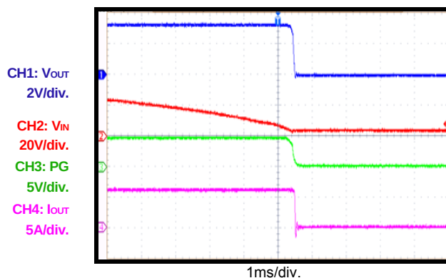
V_{IN} Shutdown
