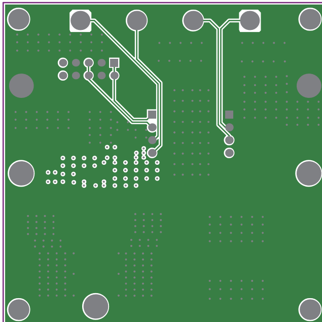
Figure 2: Mid Layer 1
