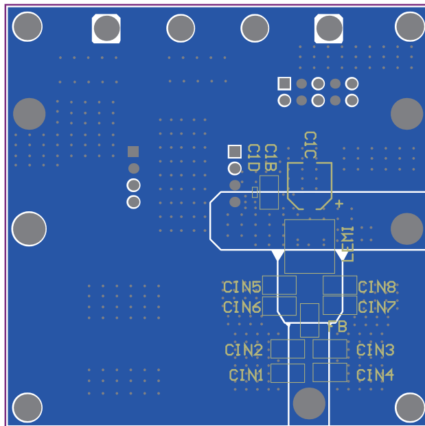
Figure 4: Bottom Layer
