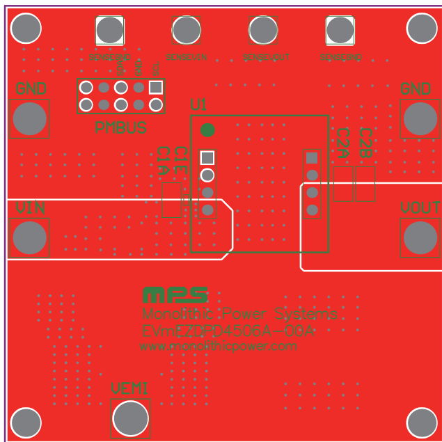
Figure 1: Top Layer
