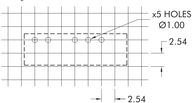
7 Pin SIP Package
