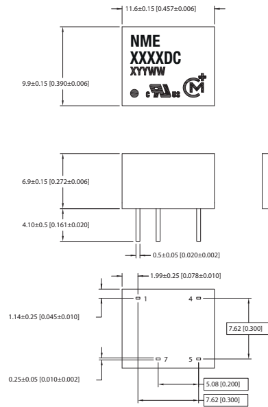
DIP Package
