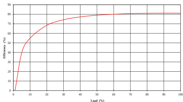
NMV0505TSAC
