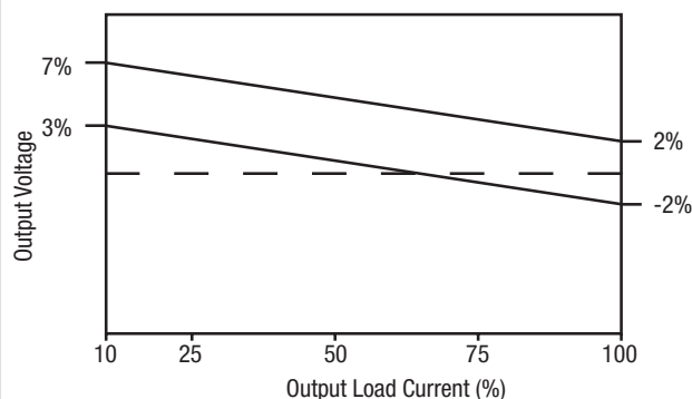
NMV0512TSC
