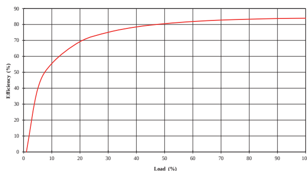
NMV0512TSC
