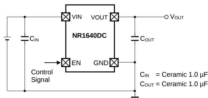
NR1640DC Typical Application Circuit
