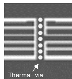
Enlarged view of IC mounting area
