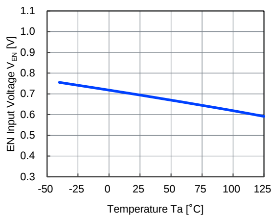
NR1640DCxxx, EN = "Low"
