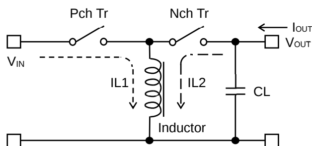
Basic Circuit
