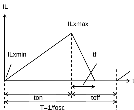
Inductor Current Waveforms (IL) through Inductor (L)
