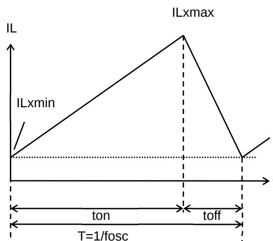
Inductor Current Waveforms (IL) through Inductor (L)
