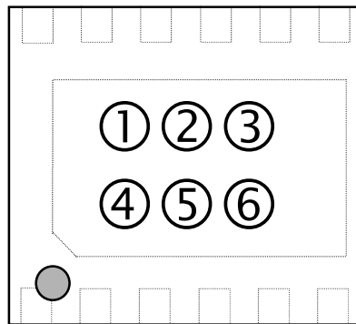
DFN(PL)2730-12 Part Markings
