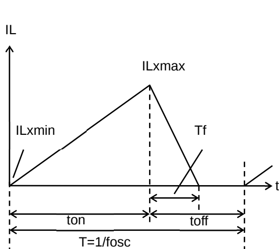
Discontinuous Inductor Current Mode
