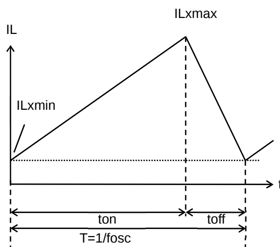
Continuous Inductor Current Mode
