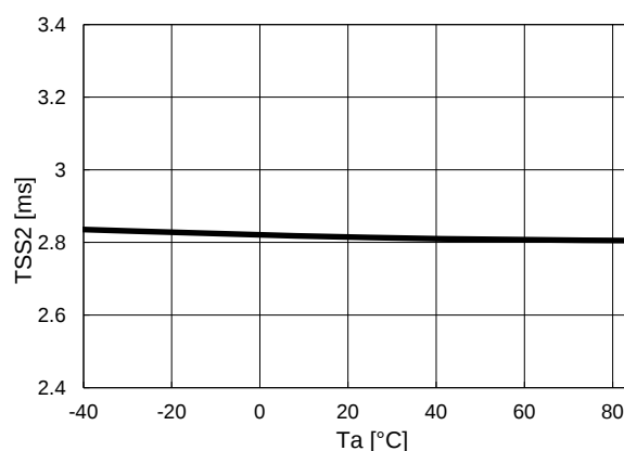
20) Delay Time for Protection vs. Temperature R1286KxxxX
