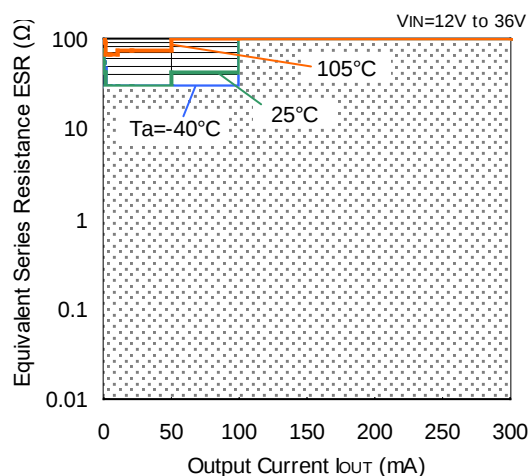
R1511x001C ( V_{OUT}=12\text{V} )
