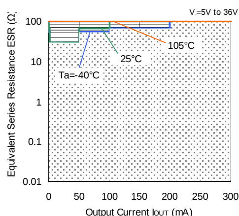
R1511x001C ( V_{OUT}=12\text{V} )
